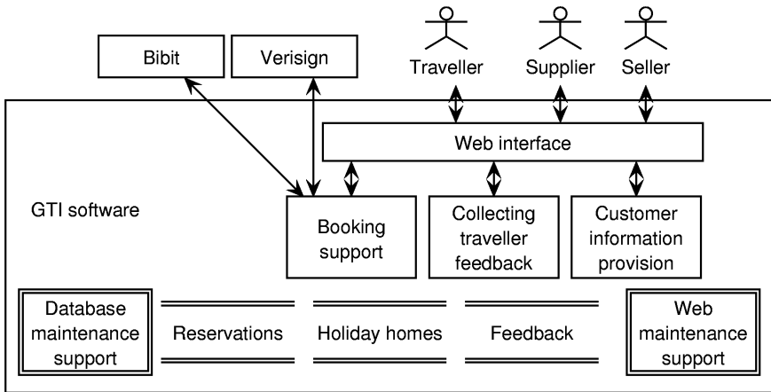
Fig. 12. Requirements-level application-architecture. Components with double borders have interfaces to all other components.
